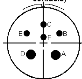
20-8 (4 #16 and 2 #8 size contacts)
