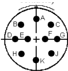
18-19 (10 #16 size contacts)
