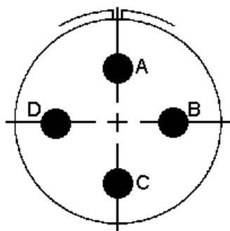
36-5 (4 #0 size contacts)
