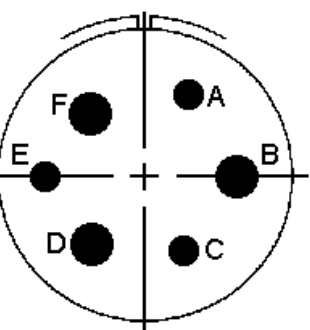
36-3 (3 #12 and 3 #0 size contacts)
