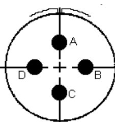
18-15 (4 #12 size contacts)
