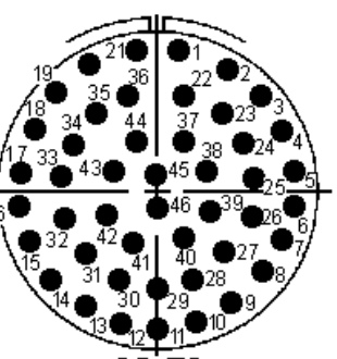
32-73 (46 #16 size contacts)
