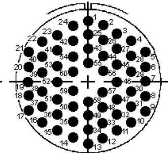
40-62 (60 #16 size contacts)
