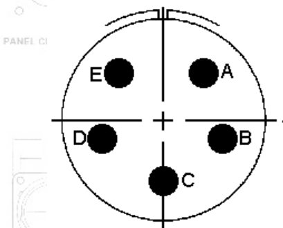
32-63 (5 #4 size contacts)
