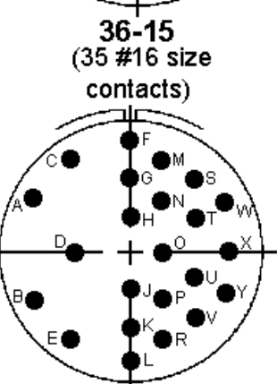
40-2 (23 #16 size contacts)
